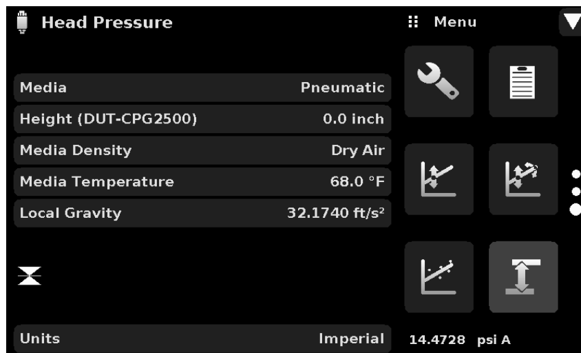
Figure 10.10-A - Head Pressure, Pneumatic
