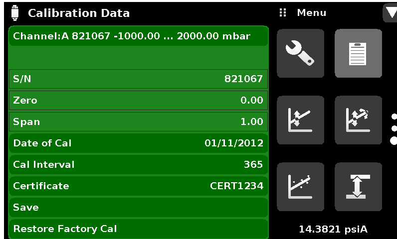
Figure 10.6 - Calibration Data
