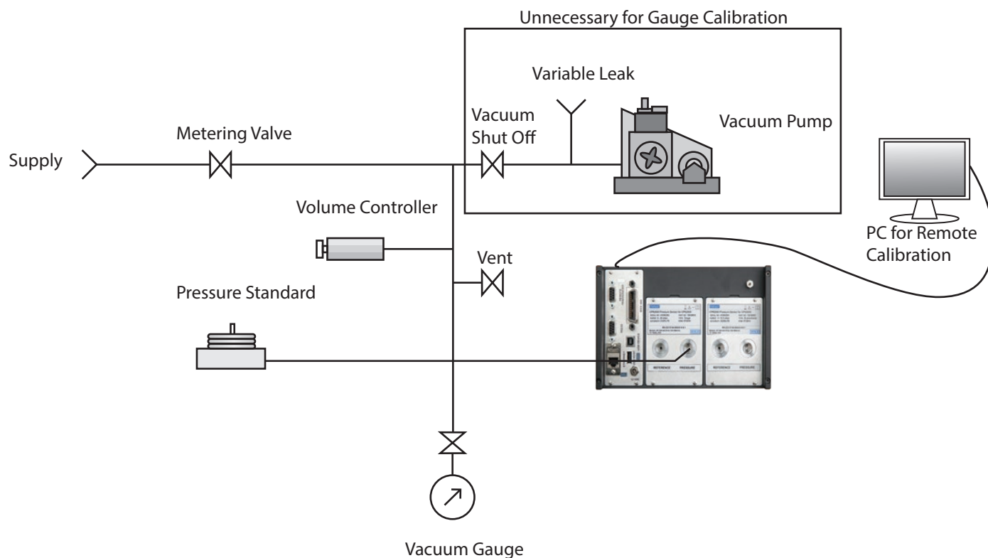
Figure 10.4 - Calibration Setup
