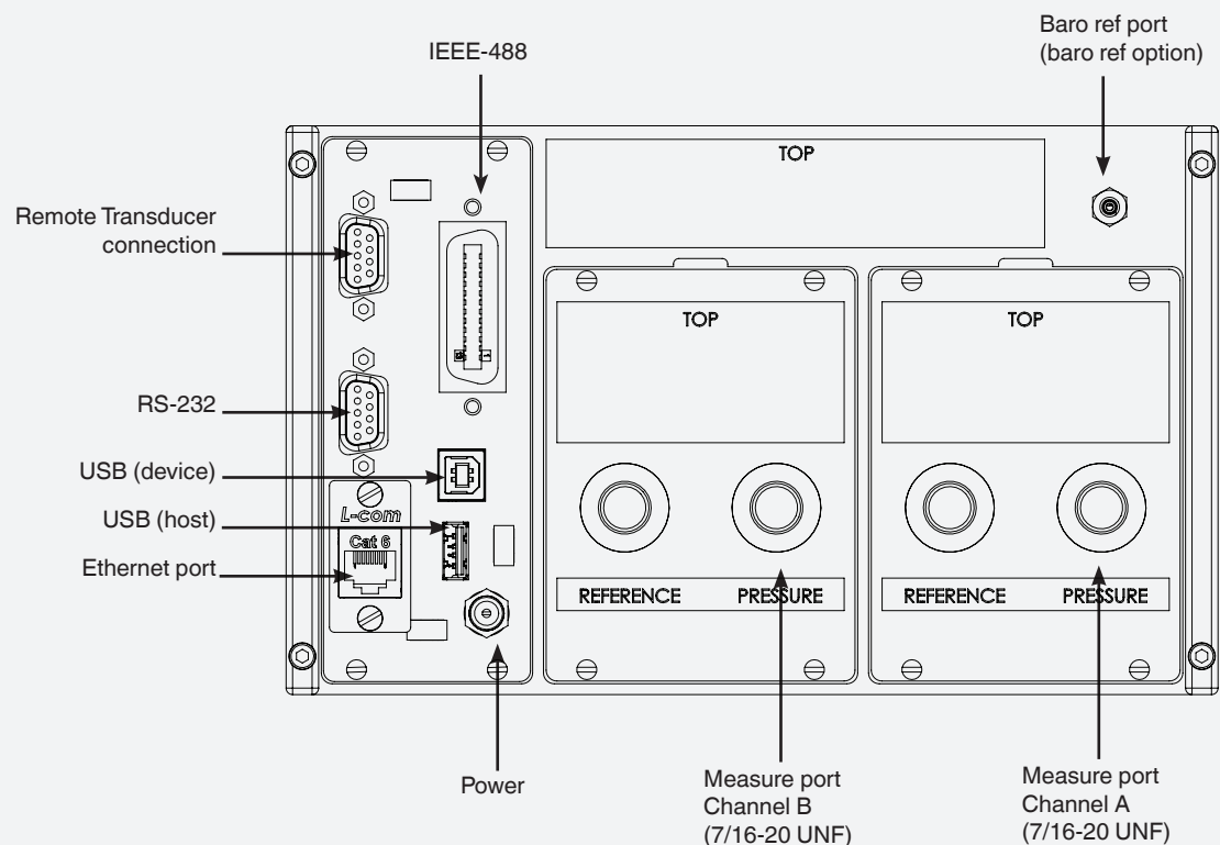
Rear Panel
